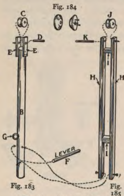
FIG. 183.—Detail of Mast.
